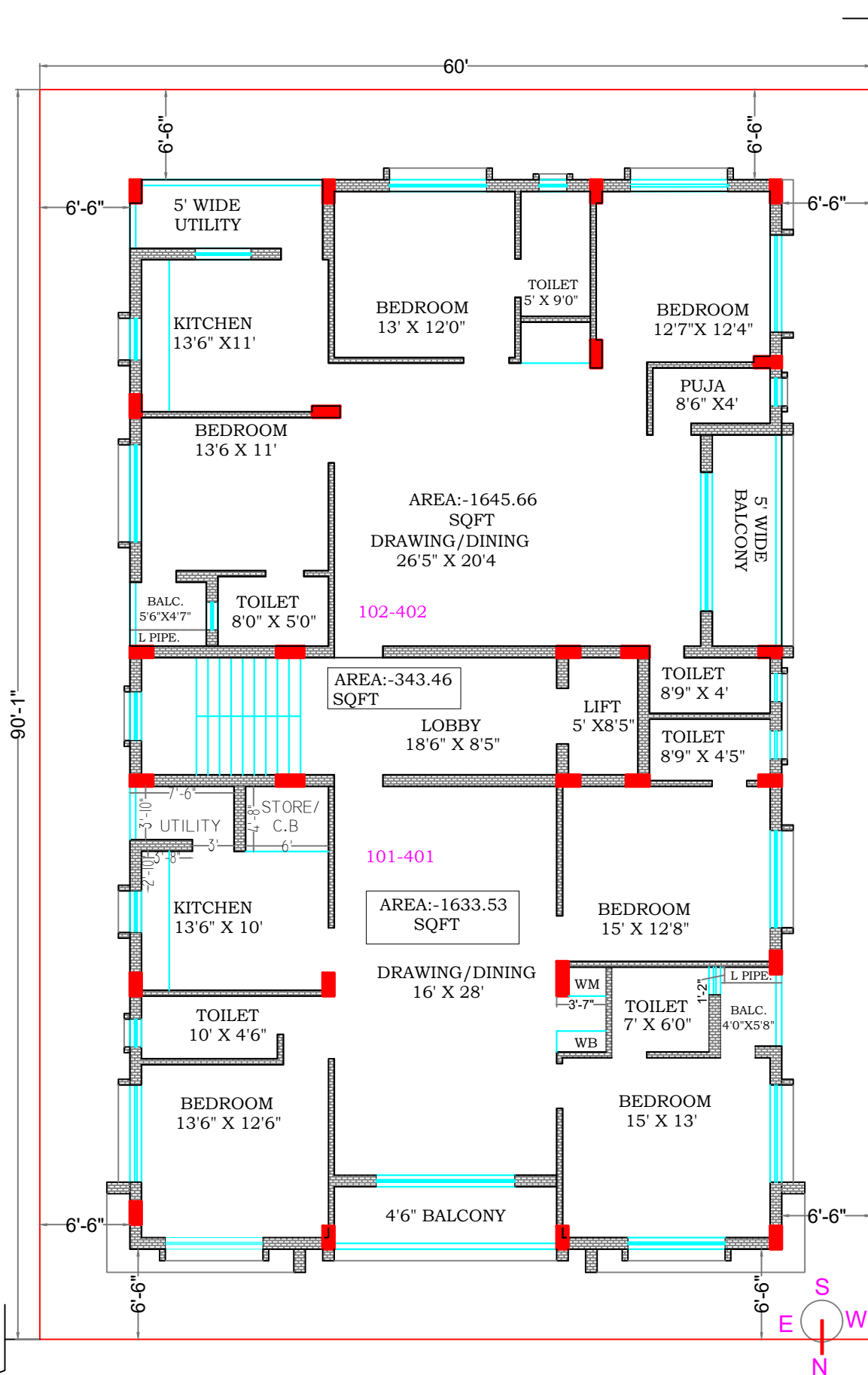
TYPICAL(1ST,2ND,3RD & 4TH)FLOOR FOR KALINGANAGAR.
